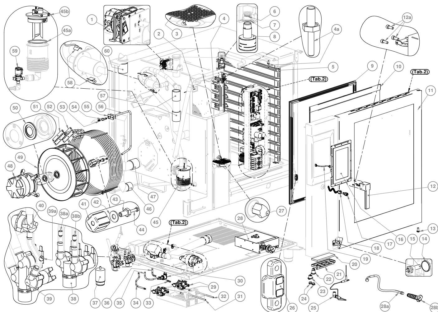
Exploded view 1/2
