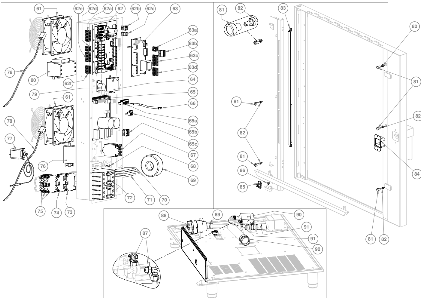
Exploded view 2/2
